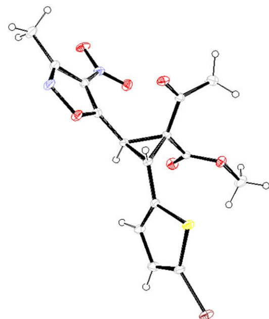
Figure 6. ORTEP representation of crystal structure of dihydrofuran 11f ; only one of the two enantiomers was shown for clarity (thermal ellipsoids are drawn at 30% probability).
