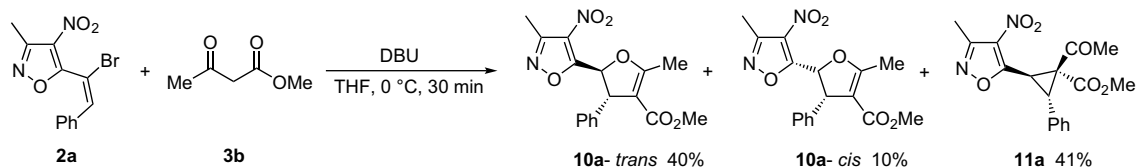
Scheme 2. Reaction of 2a and methyl acetoacetate 3b .
