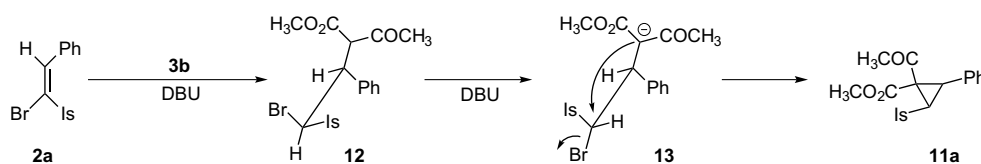
Scheme 3. Proposed mechanism for the formation of 11a .
