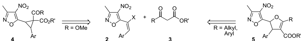
Figure 2. Retrosynthetic analysis for cyclopropanes 4 and dihydrofurans 5 .
