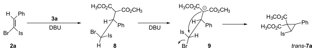
Scheme 1. Proposed mechanism for the formation of trans -7a.
