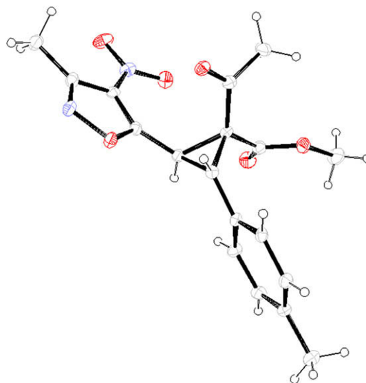
Figure 5. ORTEP representation of crystal structure of dihydrofuran 11b ; only one of the two enantiomers was shown for clarity (thermal ellipsoids are drawn at 30% probability).
