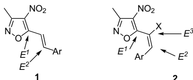
Figure 1. Polyfunctional scaffolds 1 and 2 .
