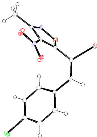
Figure 3. ORTEP representation of crystal structure of 2d (thermal ellipsoids are drawn at 30% probability).
