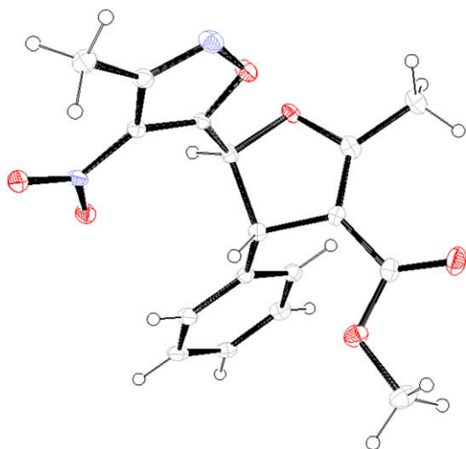
Figure 4. ORTEP representation of crystal structure of dihydrofuran 10a (thermal ellipsoids are drawn at 30% probability).
